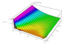
Fig.1a). 3DPlot of the Progress of Carbonation in in Semi-cylindrical Shell
